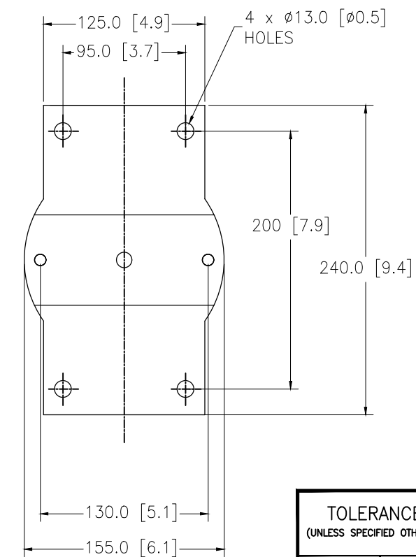
VIEW ON A-A
